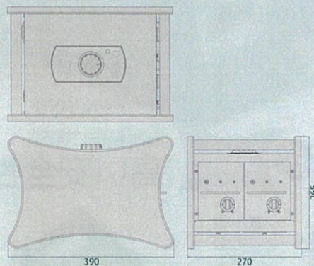
GWN-2800TW
